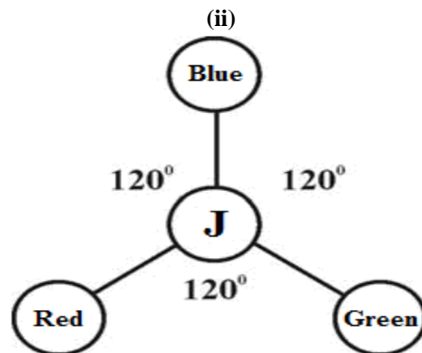
(SUPER SYMMETRY)
