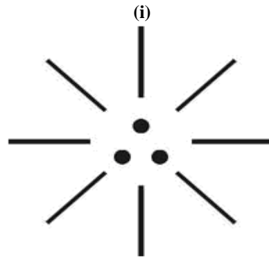
(THREE DOMAIN)
