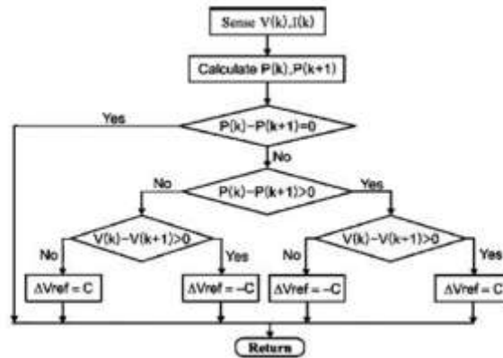
Figure 2.P & O MPPT Algorithm
