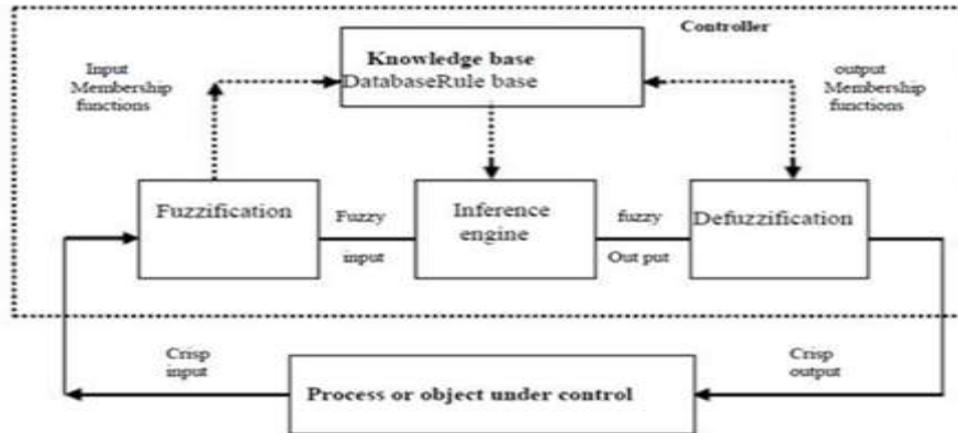
Figure 4. Fuzzy logic controller I (basic model)
