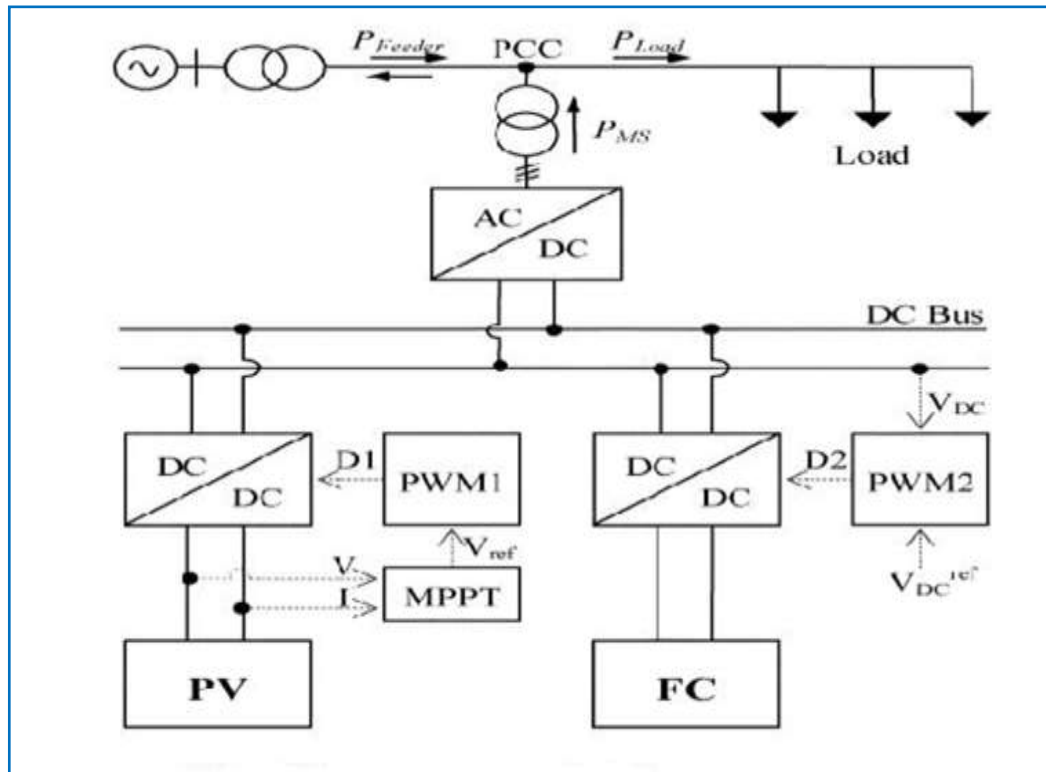
Figure 1. Grid connected PV-FC hybrid system
