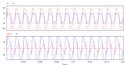
Fig: 5(b) Waveforms: Vs & Vp.
