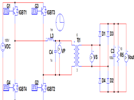
Fig:6(a) Full bridge resonance inverter(lead)
