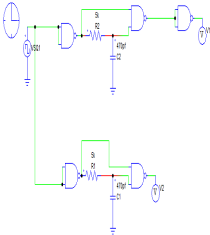
Fig: 4(c) Dead Band Circuit
