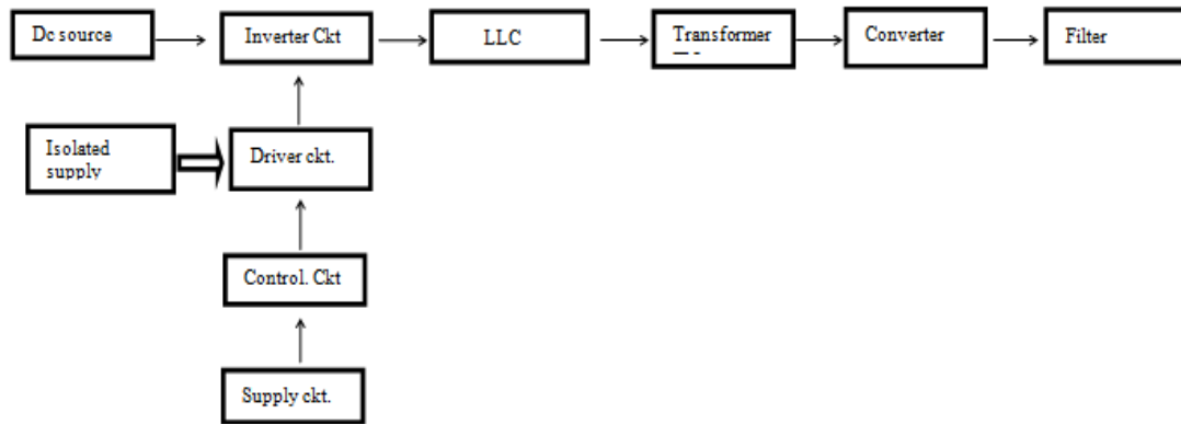
Fig: 1 Block Diagram of Resonant Frequency Converter Using Tank Circuit [5]
