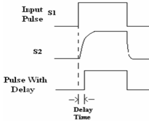
Fig: 4(b) Waveforms Of Dead Time Generator.
