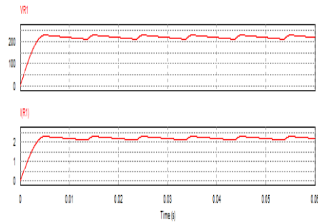
Fig: 2(b)Waveform: VR1-Up to 200V & IR1- Up to 2A
