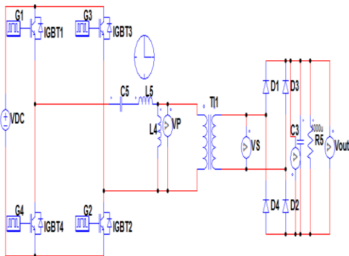
Fig: 2(e) Basic Converter design with 5kHz freq. Wave forms: Vout & Iout, where Vout=app 200V , Iout=5A
