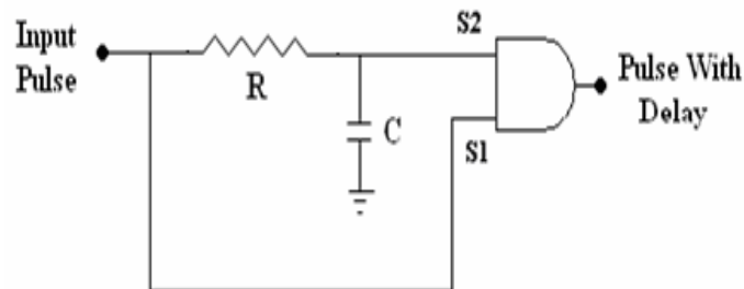
Fig: 4(a) Dead Time Generator.
