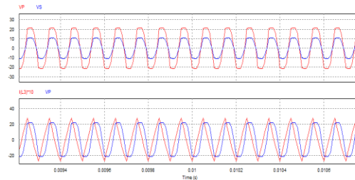
Fig: 6(b) Waveform-Vs&Vp Along With Ic and Vp.
