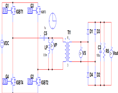
Fig: 5(a) Full bridge Lag Inverter
