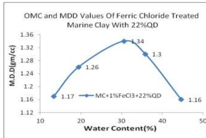
Fig. 2 (d): OMC and MDD of Quarry dust
