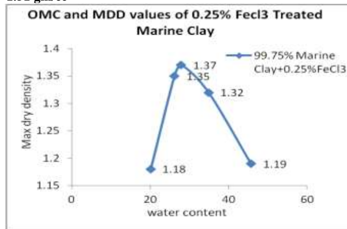
Fig. 1 (b): OMC and MDD of 0.25% FeCl 3 marine clay
