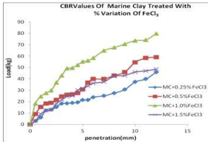
Fig.3: CBR Value of marine clay with FeCl 3
