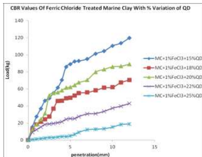
Fig.3: CBR Value of marine clay with Quarry dust
