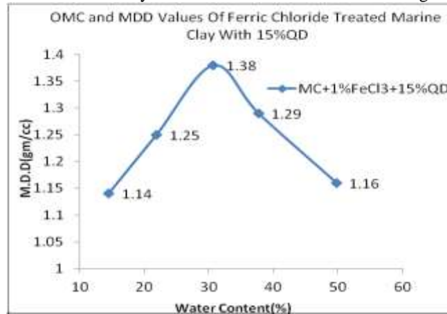
Fig.2 (a): OMC and MDD of Quarry dust
