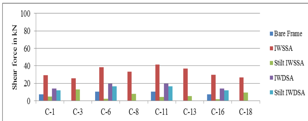
Fig. (b) Shear Forces (Dynamic Analysis) in Columns for 6.0 m bottom storey height
