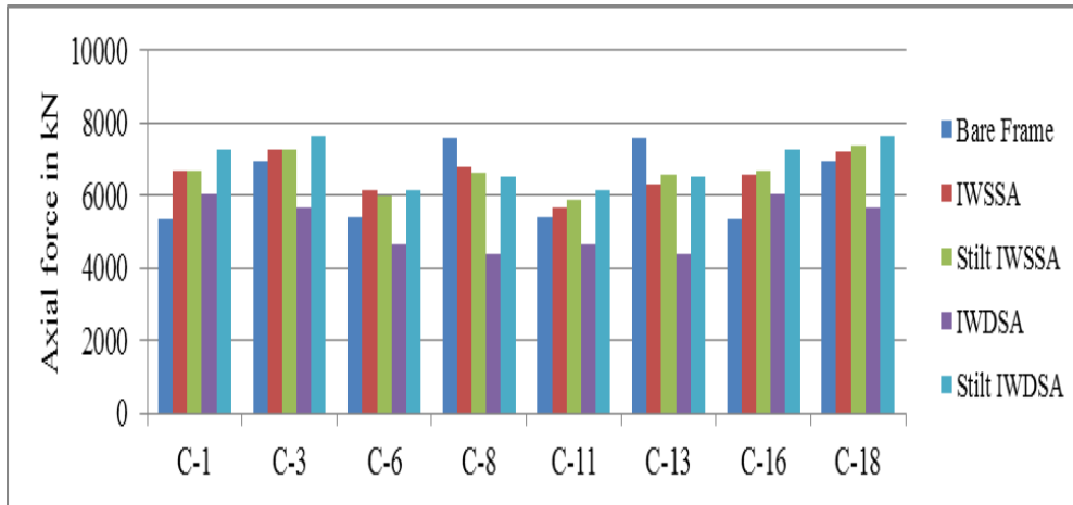
Fig. (b) Axial Forces (Dynamic Analysis) in Columns for 4.5 m bottom storey height
