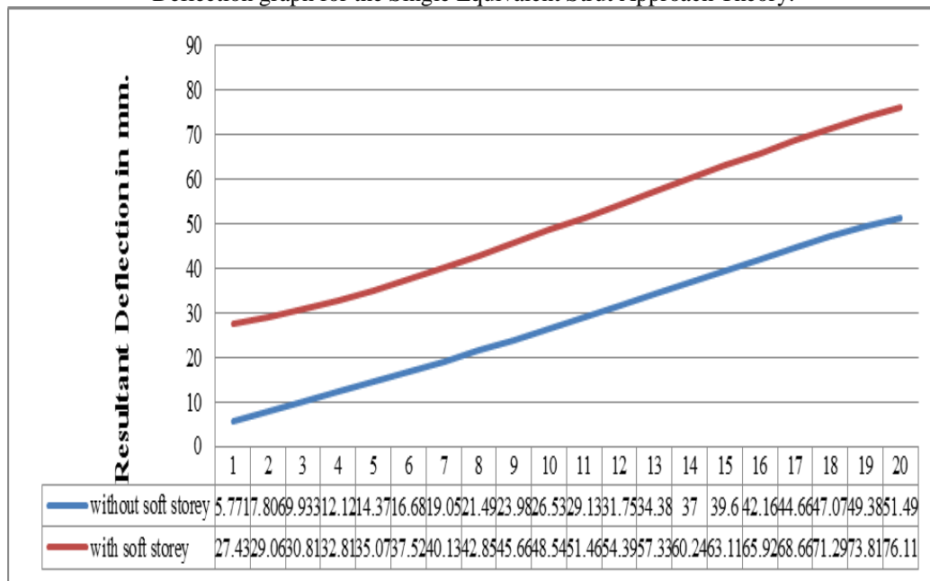
Fig. (a) Deflection for Static Analysis for 6.0 m bottom storey height
