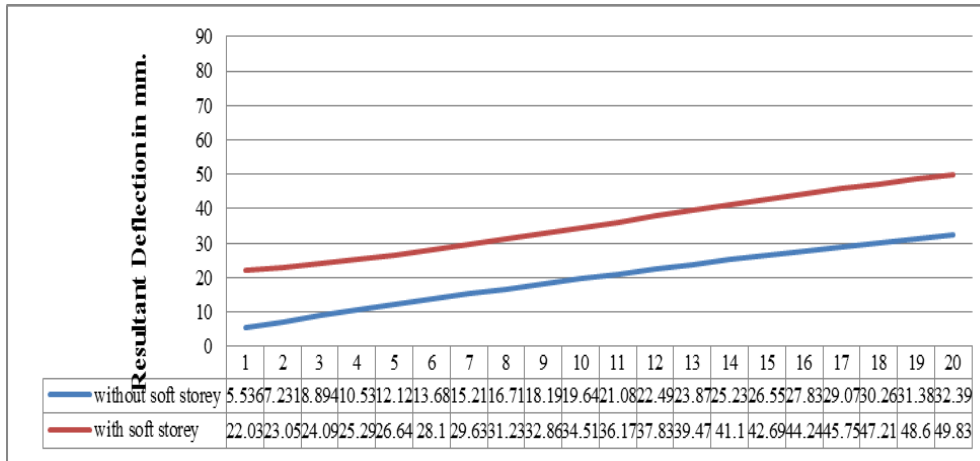
Fig. (b) Deflection for Dynamic Analysis for 6.0 m bottom storey height
