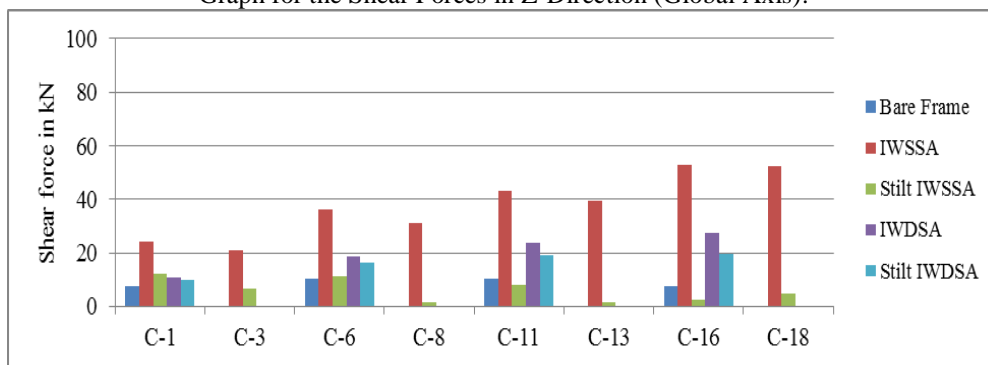
Fig. (a) Shear Forces (Static Analysis) in Columns for 6.0 m bottom storey height
