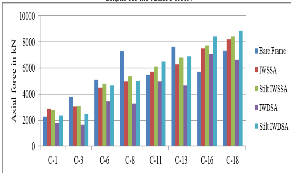
Fig. (a) Axial Forces (Static Analysis) in Columns for 4.5 m bottom storey height
