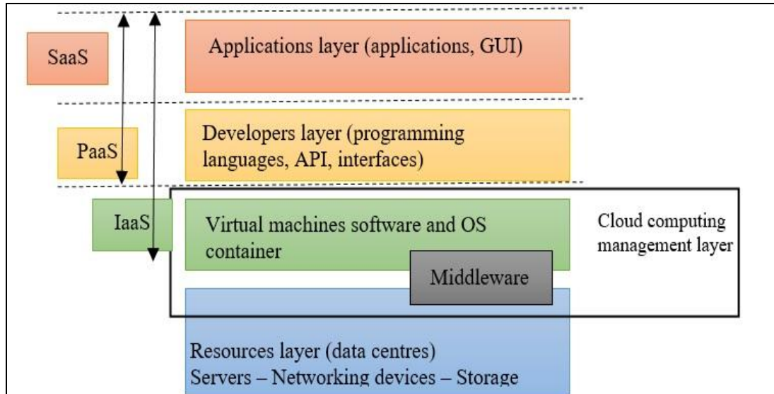
Fig.7: A cloud computing architecture showing the available services for each delivery model. Infrastructure as a service (IaaS) has low level access. Platform as a service (PaaS) provides development tools and interfaces. Software as a service (SaaS) is completed tools and capabilities.
