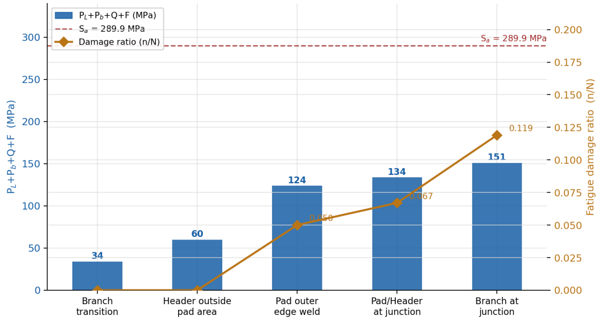
Figure 4: Fatigue stress P_L + P_b + Q + F and damage ratio (n/N) at FE/Pipe named locations. 7,000 design cycles; S_a = 289.9 MPa. Maximum damage ratio = 0.119 at branch junction. All locations Code-compliant.
