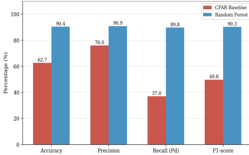
Figure 3. Random Forest vs. CFAR Baseline Performance on the Simulated Test Set
