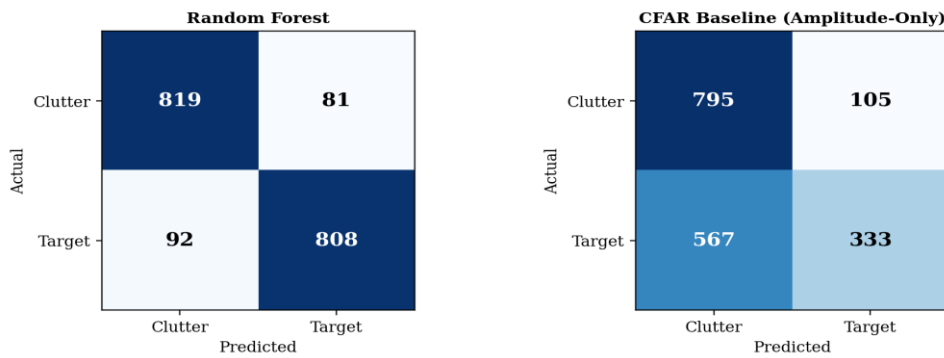
Figure 4. Confusion Matrices – Random Forest and CFAR Baseline (Test Set, n = 1,800 )
