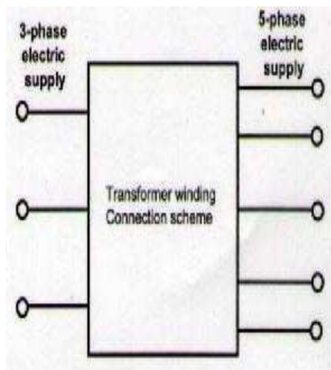
Fig. 1. Block representation of the proposed system.
