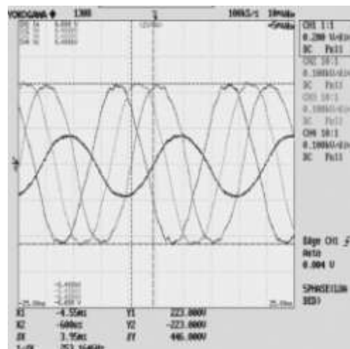
Fig. 9. Output side (five-phase) voltages and current waveform.
