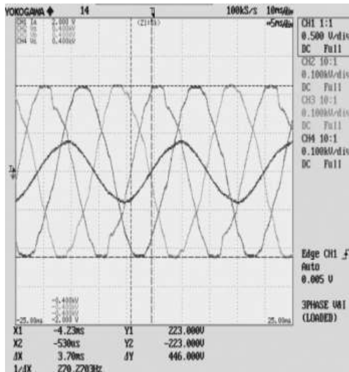
Fig. 8. Input side (three-phase) voltages and current waveform.
