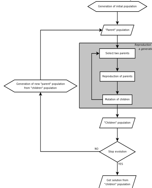
Fig 3. Flow Diag. for Genetic Algorithm
