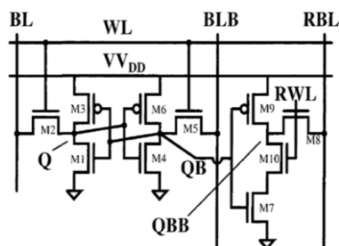
Figure 4. 10T SRAM cell
