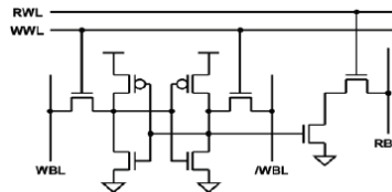
Figure 2. 8T SRAM Cell
