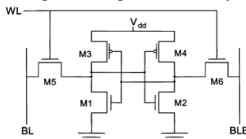
Figure 1. Conventional 6T SRAM
