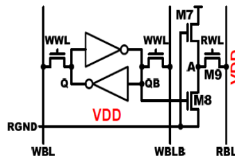
Figure 3. 9T SRAM Cell
